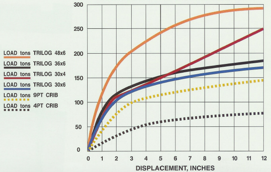
NIOSH SAFETY STRUCTURES WOOD CRIB TESTS
